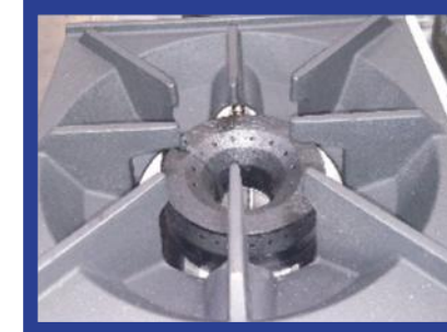
Slope design guides spills away from burner ports with integrated pilot protector
